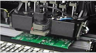
Fiducial Camera (2D) For Board Barcode Scanning
