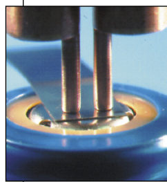
88A/EZ Precision Weld Head
